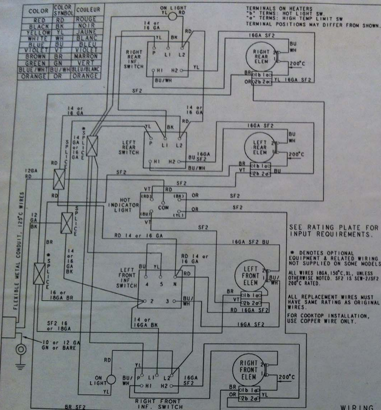
WIRING DIAGRAM
