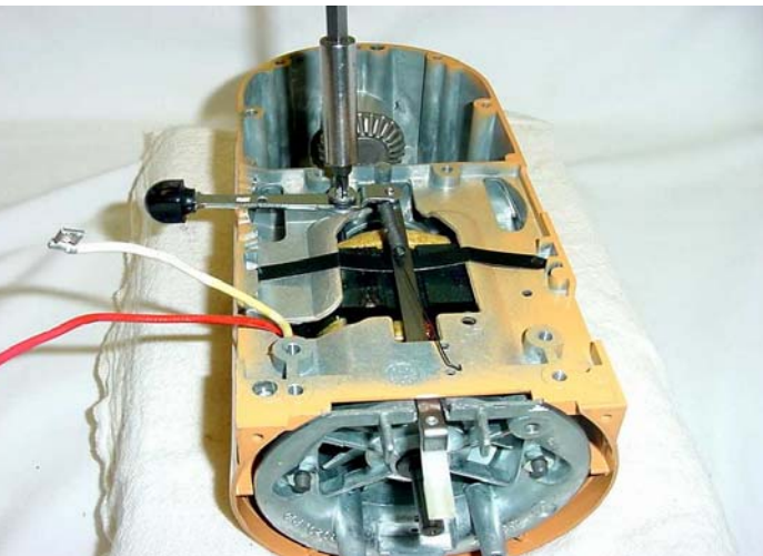
Fig. 44 Securing the pivot screw to the gearcase after placing the tension washer.
