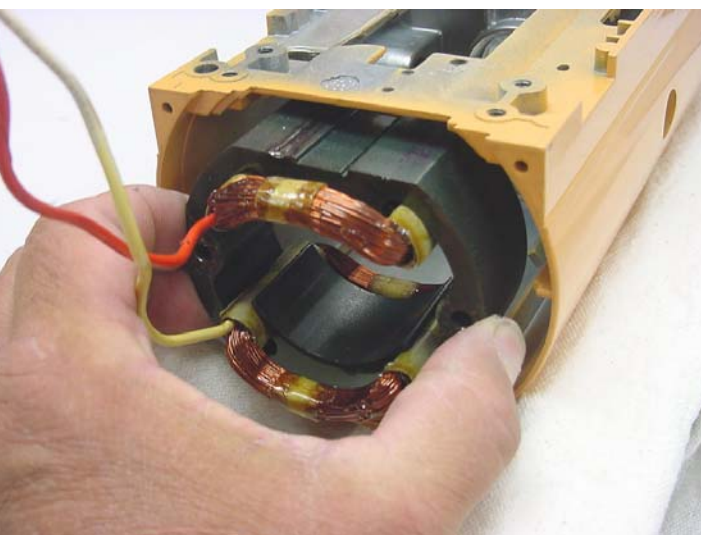
Fig. 32 The stator is shown being removed from the motor housing.
