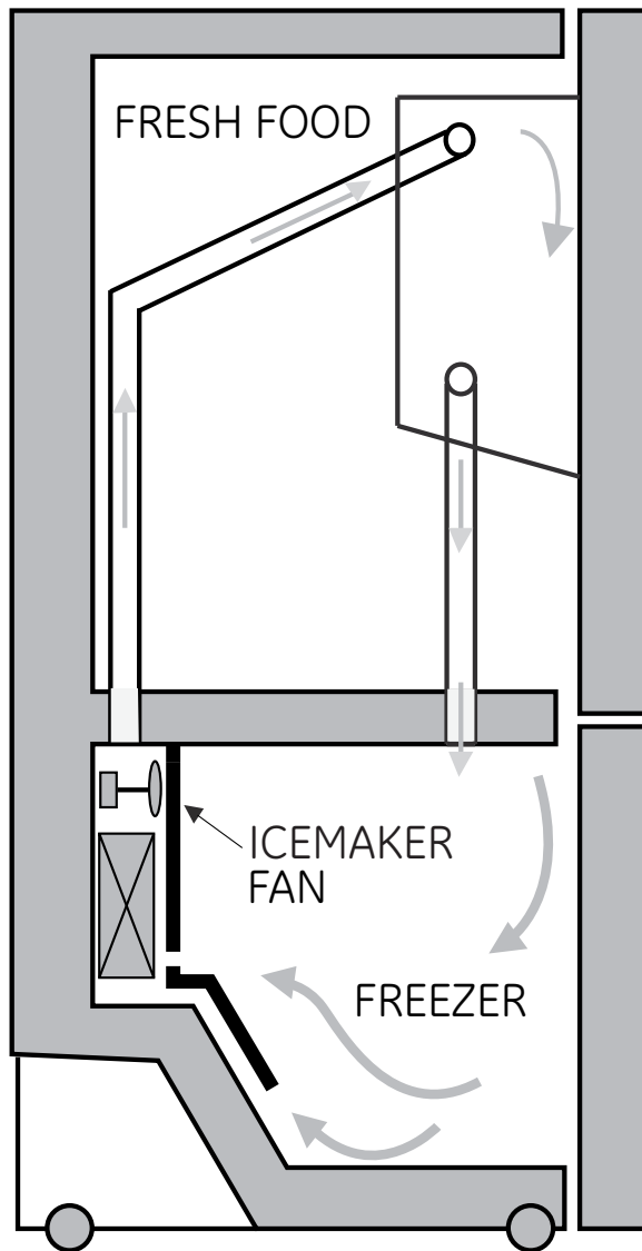
Ice System Air Flow (side view)
