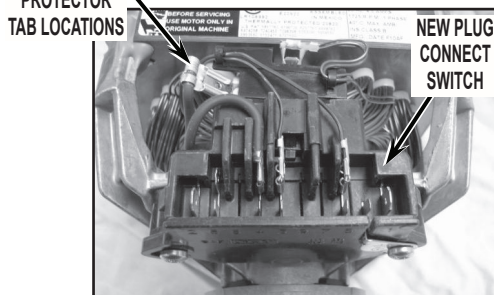
FIGURE 2C (REPLACEMENT MOTOR)
