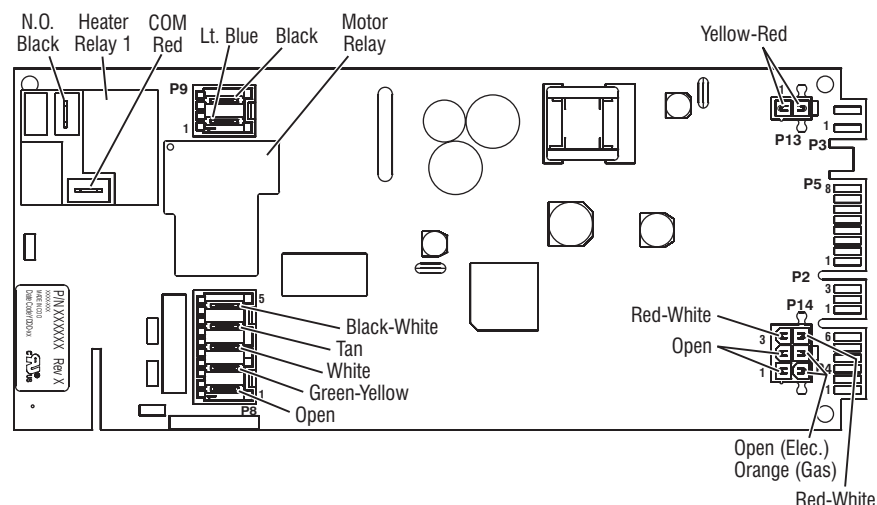
Figure 17. Machine control electronics.
