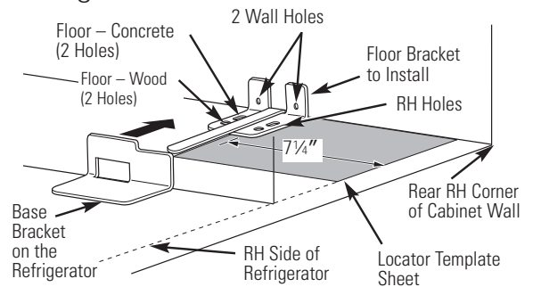
Figure 1 – Installation Overview
