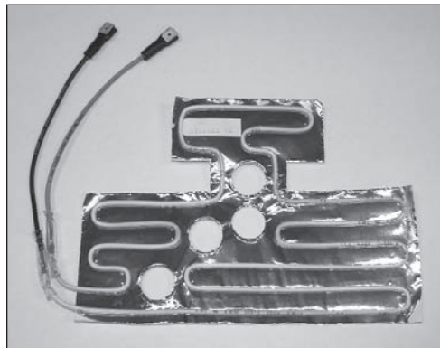
Heater Kit
