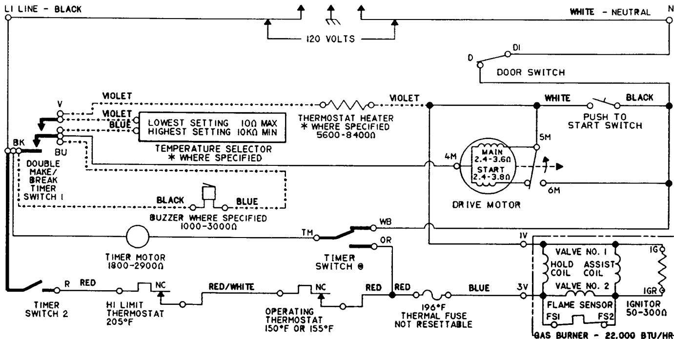
PLUGGABLE DRIVE MOTOR SWITCH WIRING DIAGRAM
