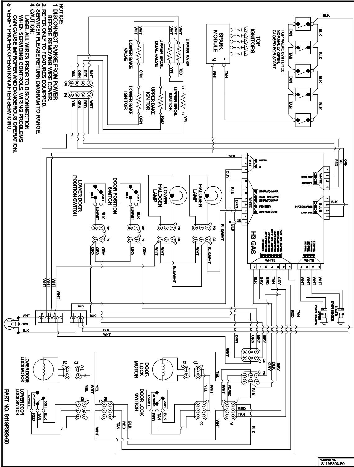
Wiring Diagram
