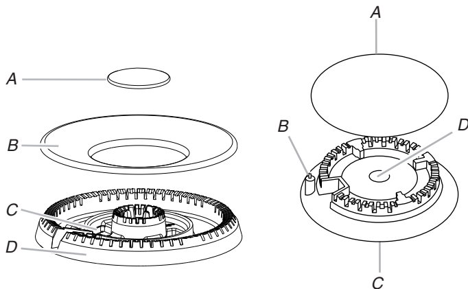
A. Inner burner cap B. Outer burner cap C. Gas tube opening D. Burner base
