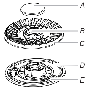
A. Inner burner cap B. Inner burner base C. Outer burner base D. Burner support E. Gas tube opening
